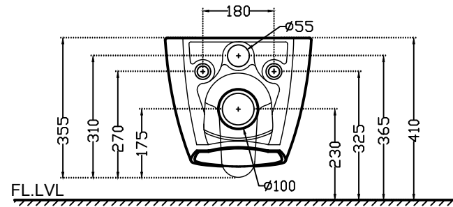
BACK VIEW
